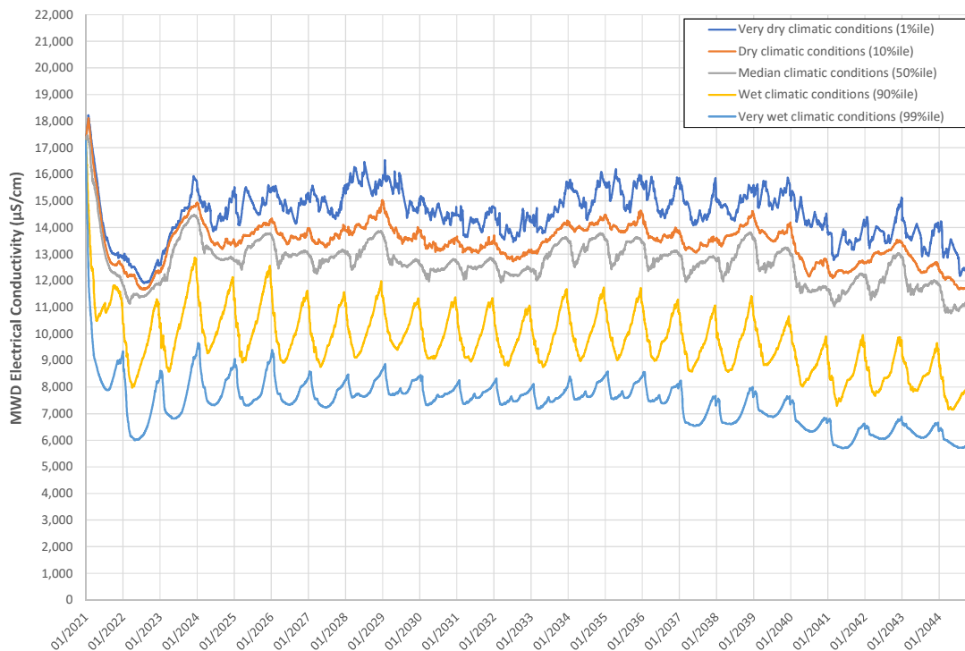
Figure 6.2 - Forecast MWD salinity
