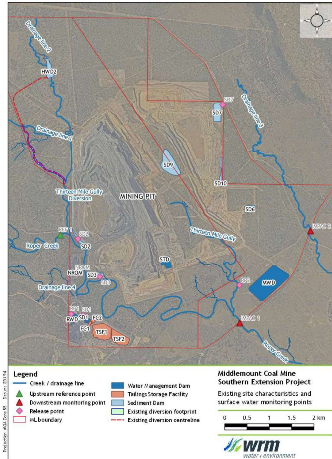
Figure 3.2 - Middlemount Coal Mine existing site characteristics and surface water monitoring locations
