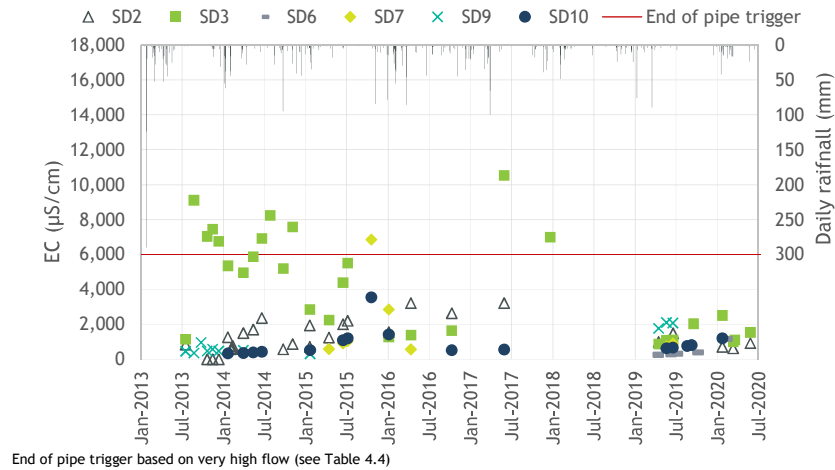
Figure A.4 - EC - On-site stormwater sediment dams
