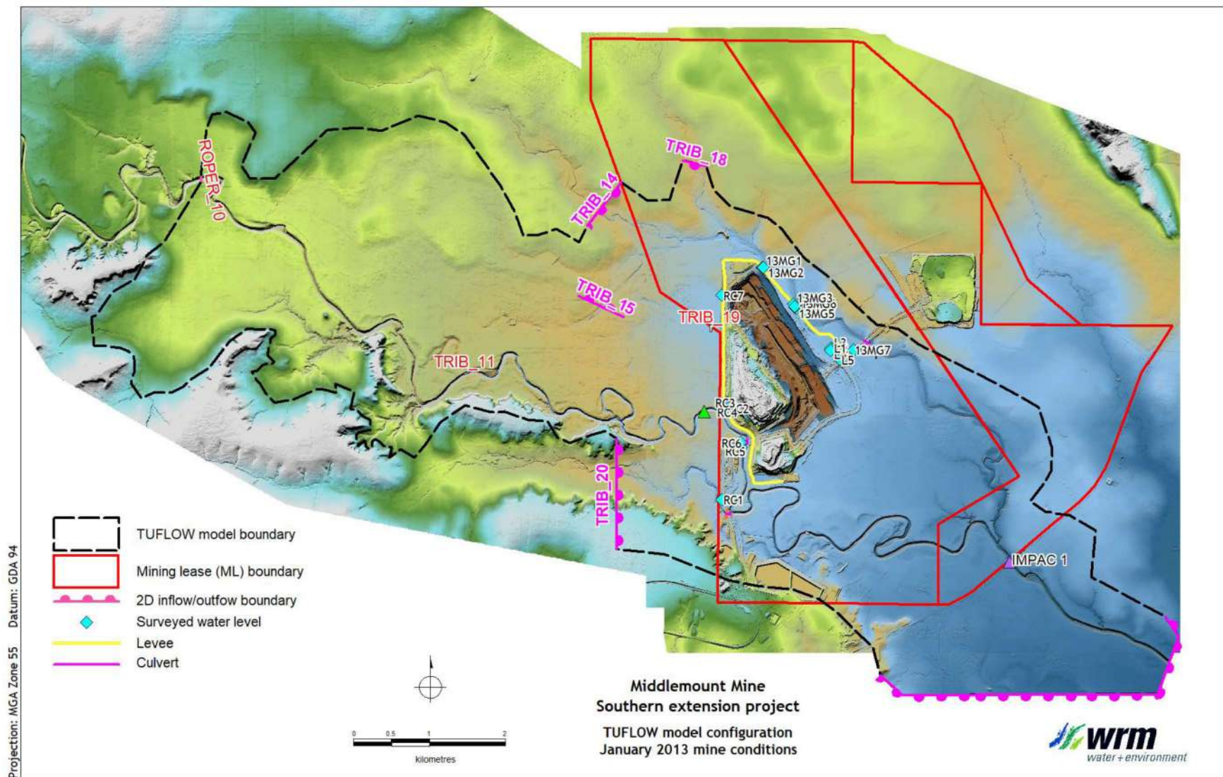
Figure 8.8 - January 2013 Roper Creek TUFLOW model configuration
