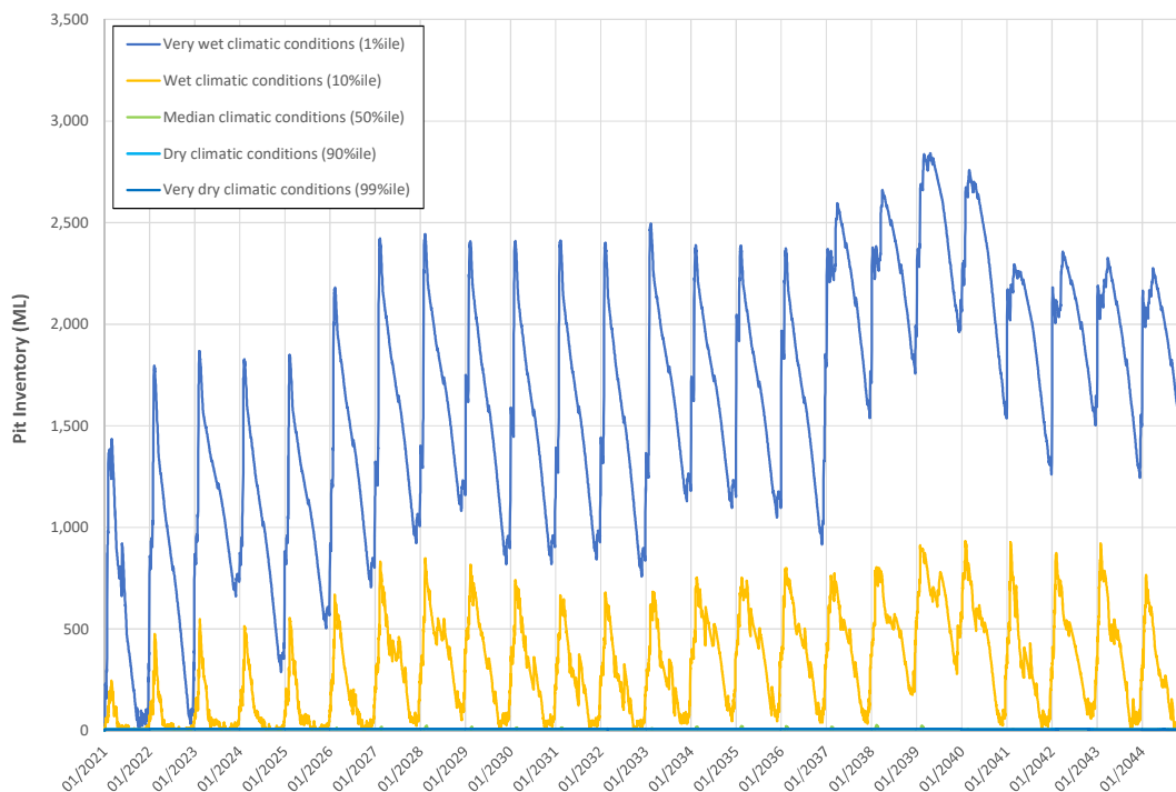
Figure 6.3 - Forecast mining pit inventory
