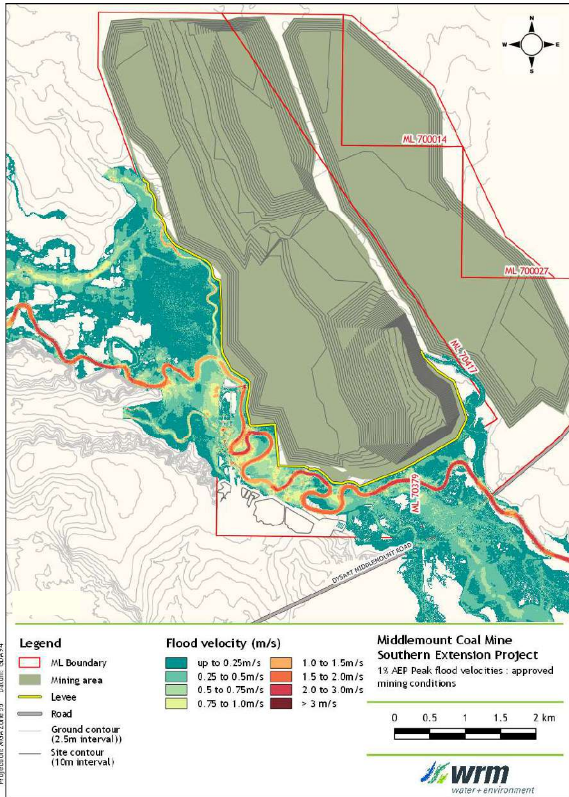
Figure 8.14 - Approved conditions flood velocities, 1% AEP event.
