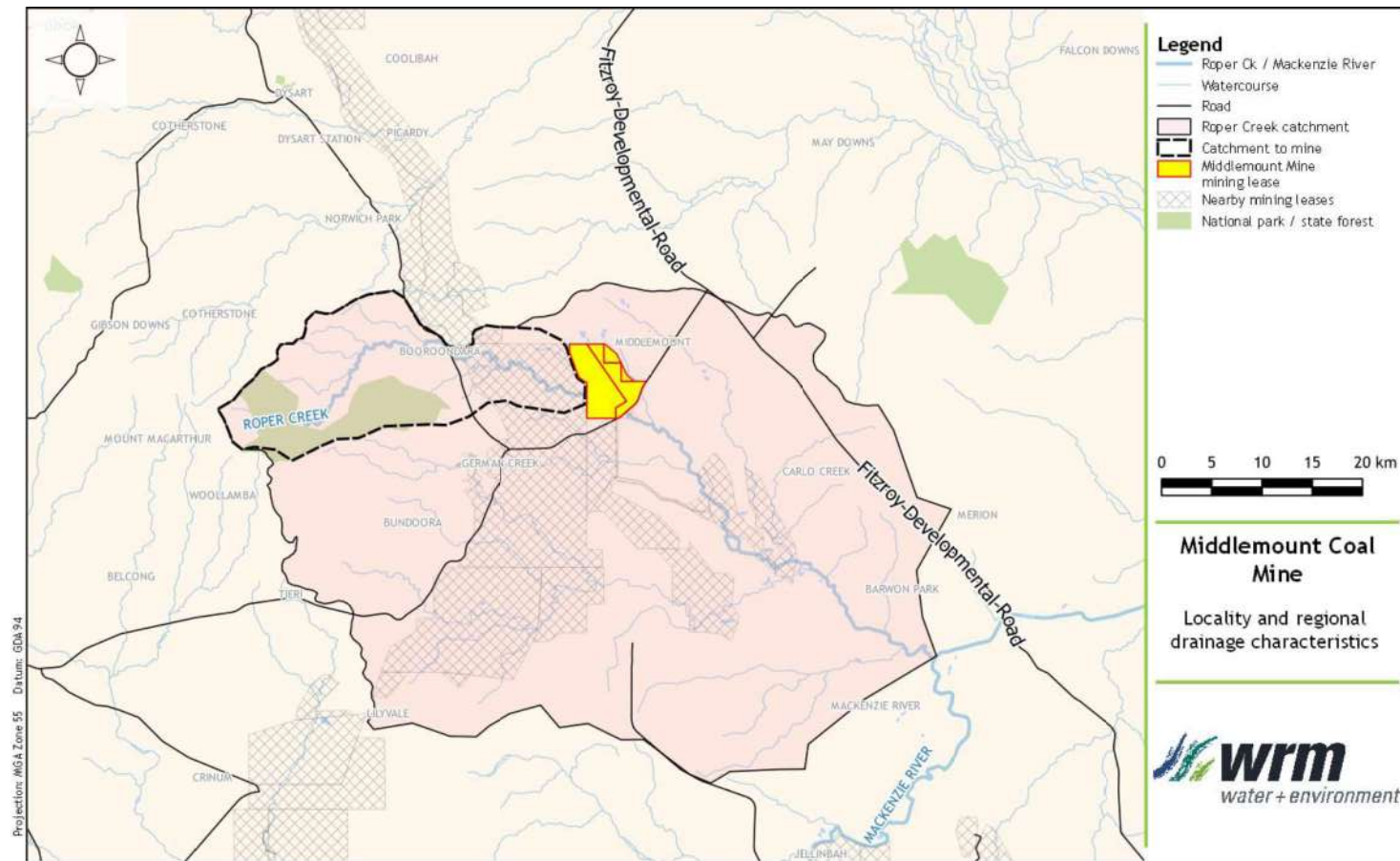
Figure 3.1 - Regional drainage characteristics
