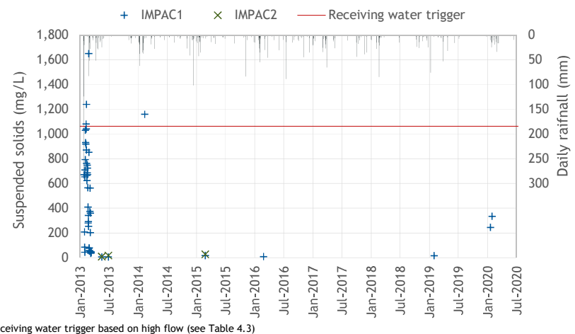
Figure A.12 - Suspended solids - Downstream surface water monitoring locations
