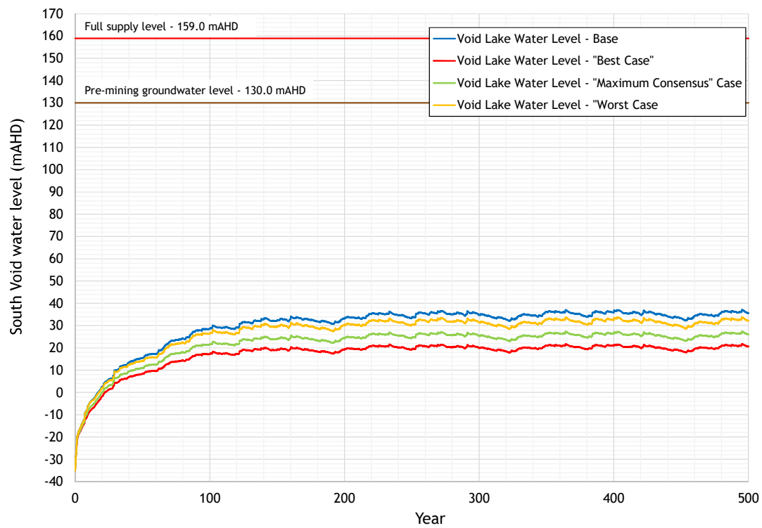
Figure 7.7 - South Void water level - climate change assessment
