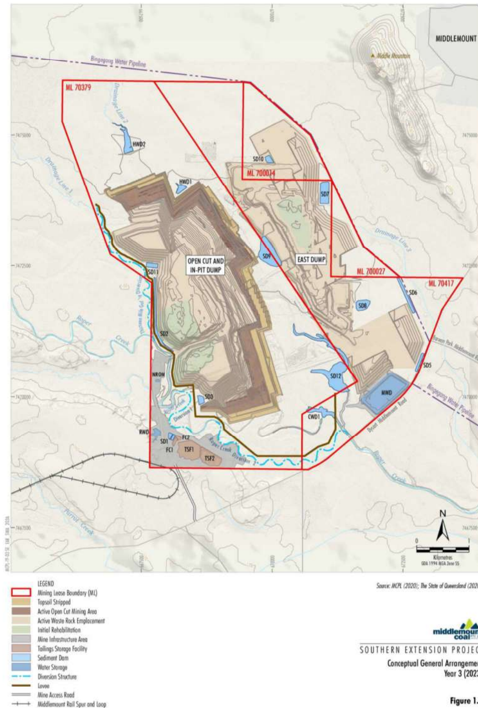
Figure 1.3 - Proposed general layout, Year 3 (2023)
