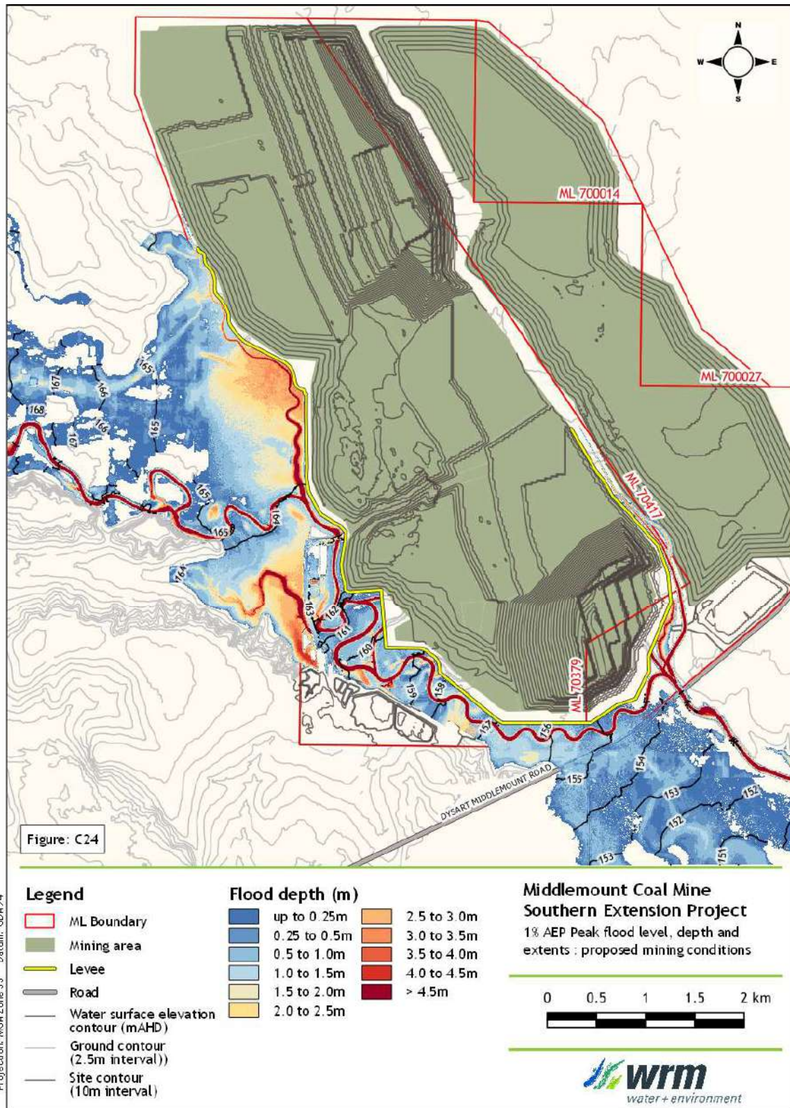
Figure 9.5 - Flood depths and extent, proposed conditions, 1% AEP
