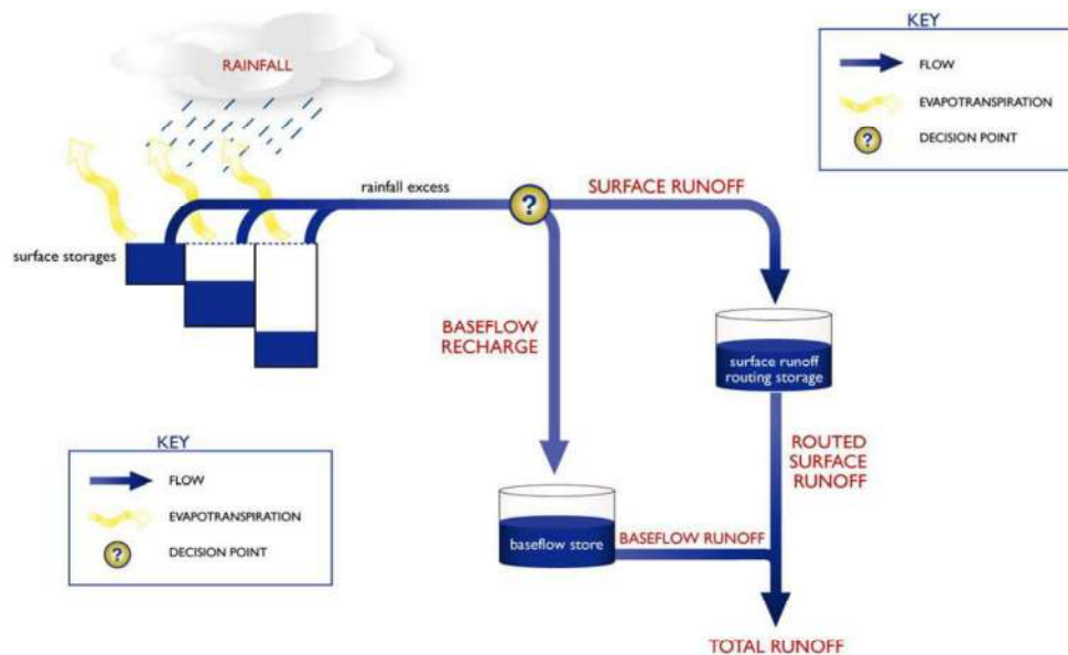
Figure B.7 - AWBM model configuration
