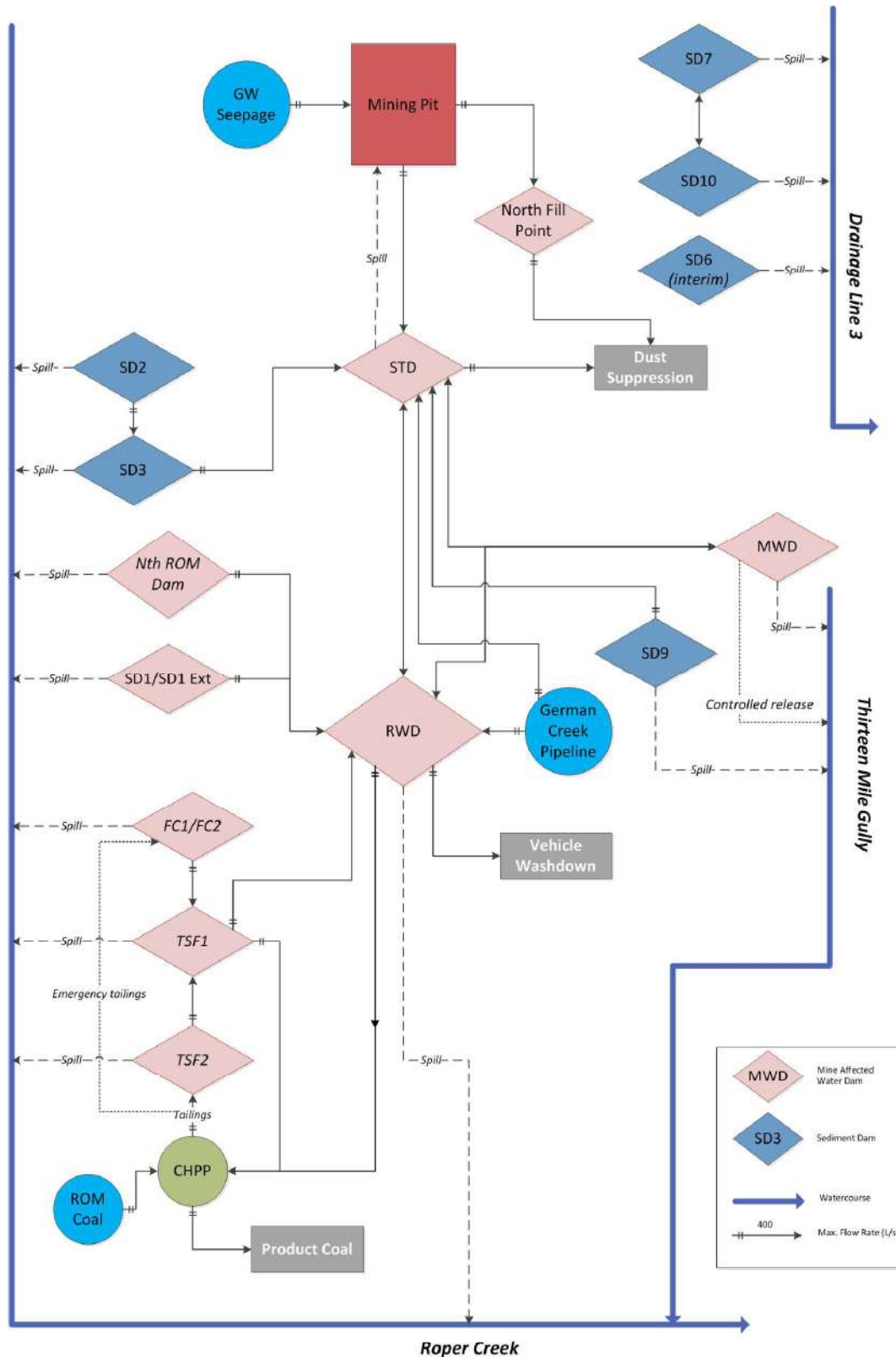
Figure 5.1 - Existing water management system schematic
