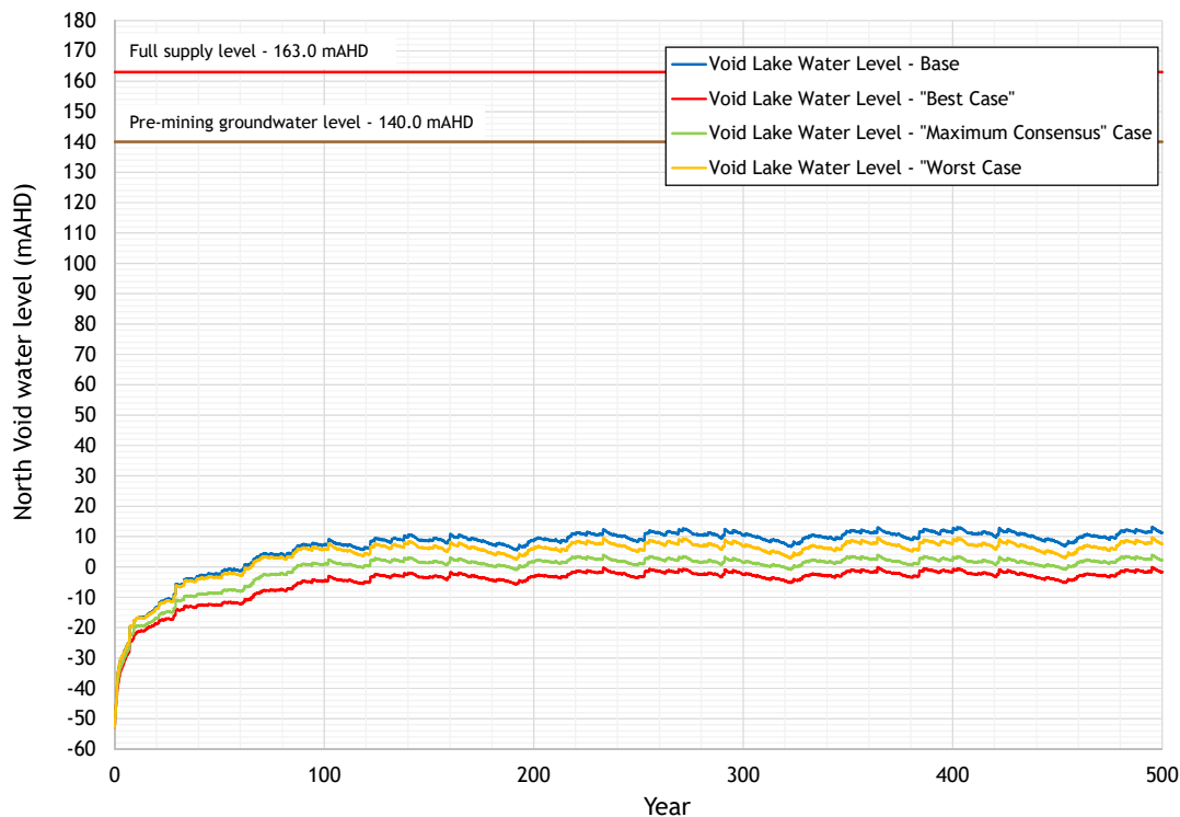
Figure 7.6 - North Void water level - climate change assessment
