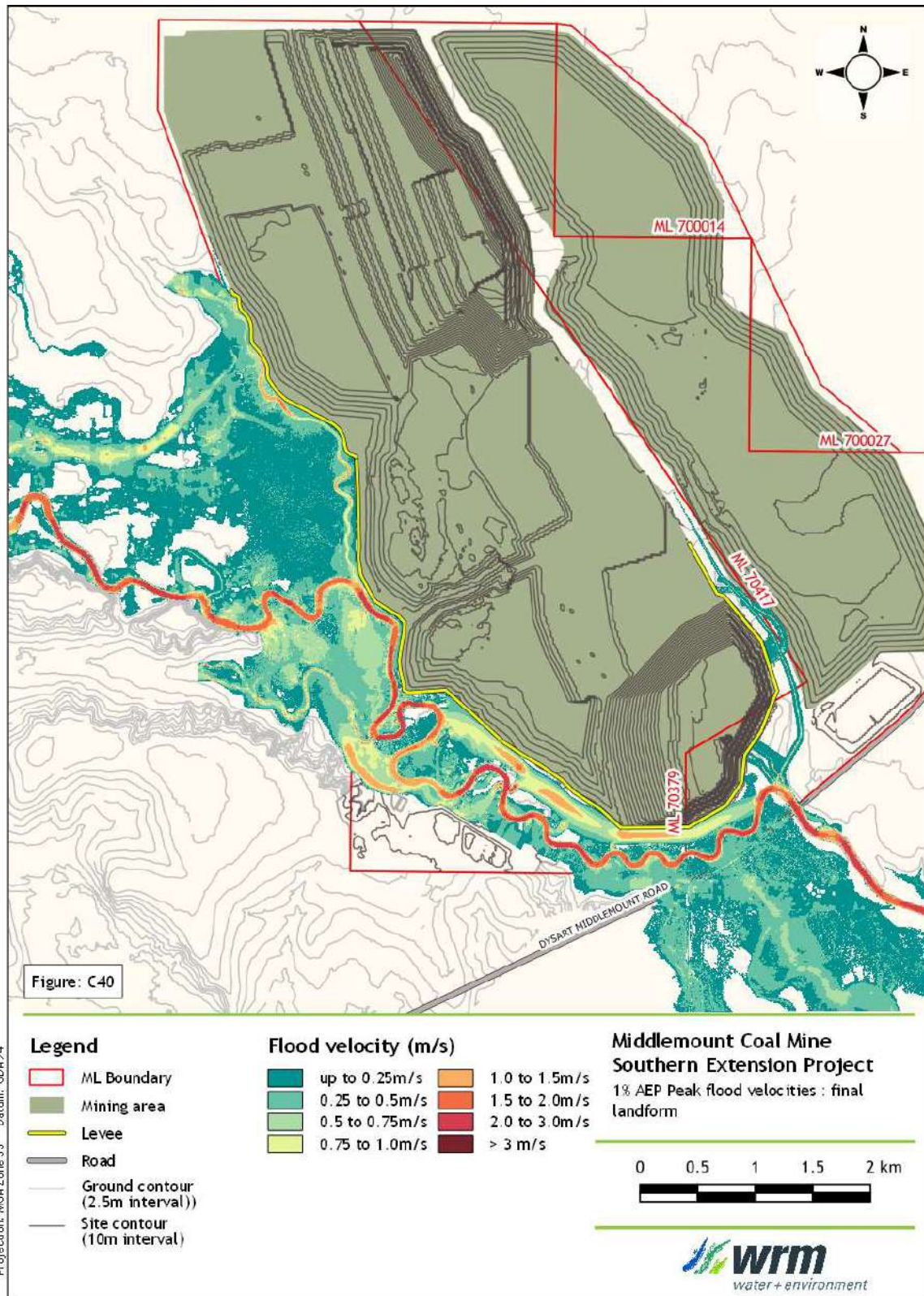
Figure 9.10 - Flood velocities, Post mining conditions, 1% AEP
