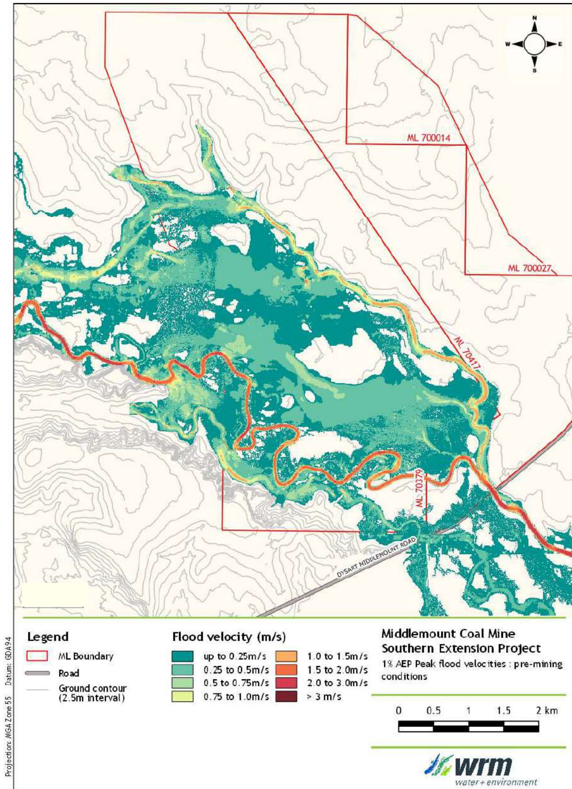
Figure 8.12 - Pre-mining conditions flood velocities, 1% AEP event.
