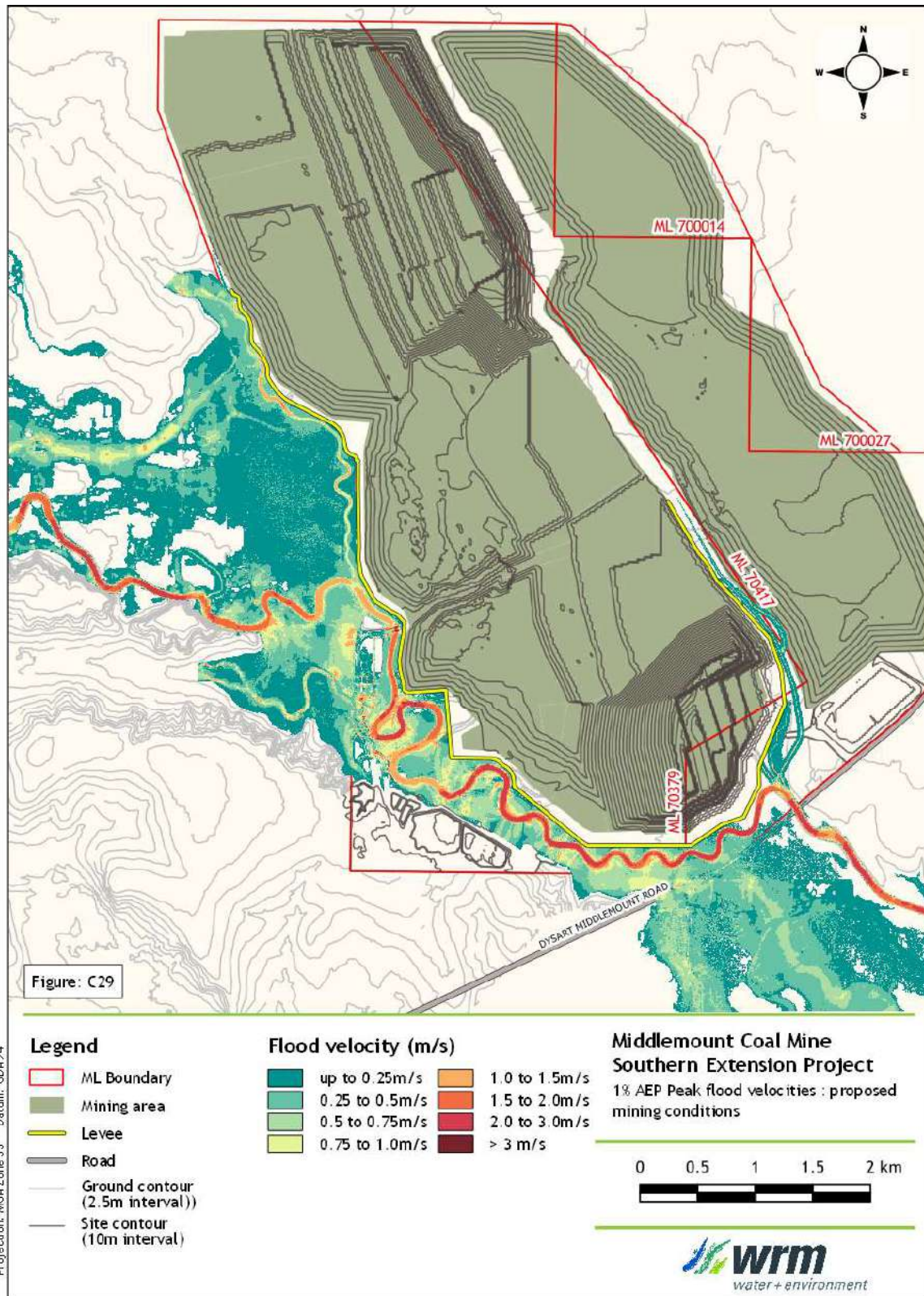
Figure 9.6 - Flood velocities, proposed conditions, 1% AEP
