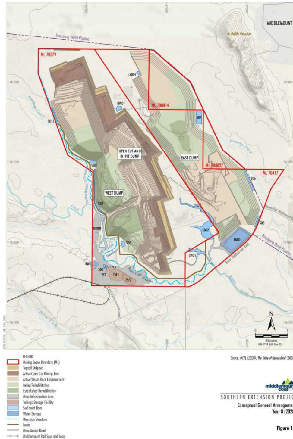
Figure 1.4 - Proposed general layout, Year 8 (2028)
