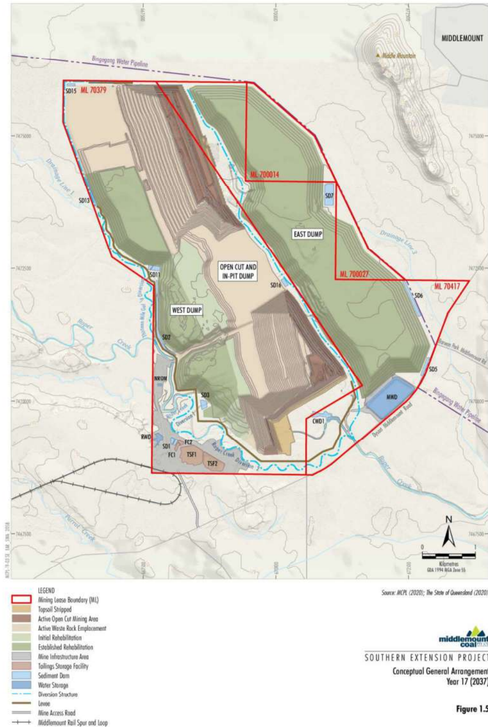
Figure 1.5 - Proposed general layout, Year 17 (2037)
