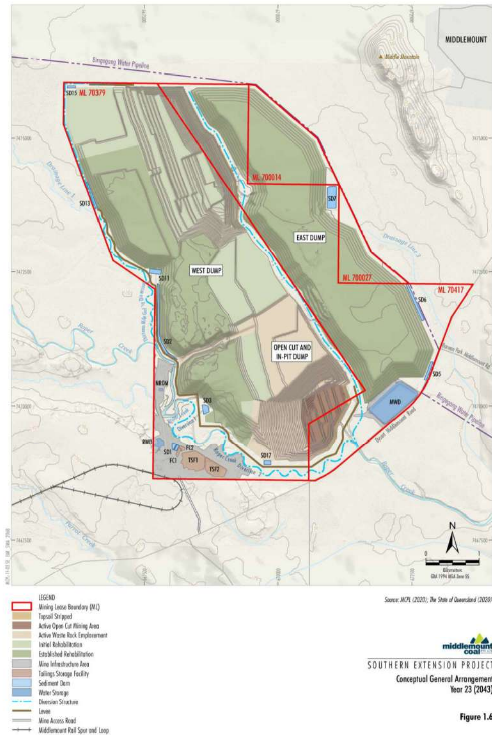
Figure 1.6 - Proposed general layout, Year 23 (2043)
