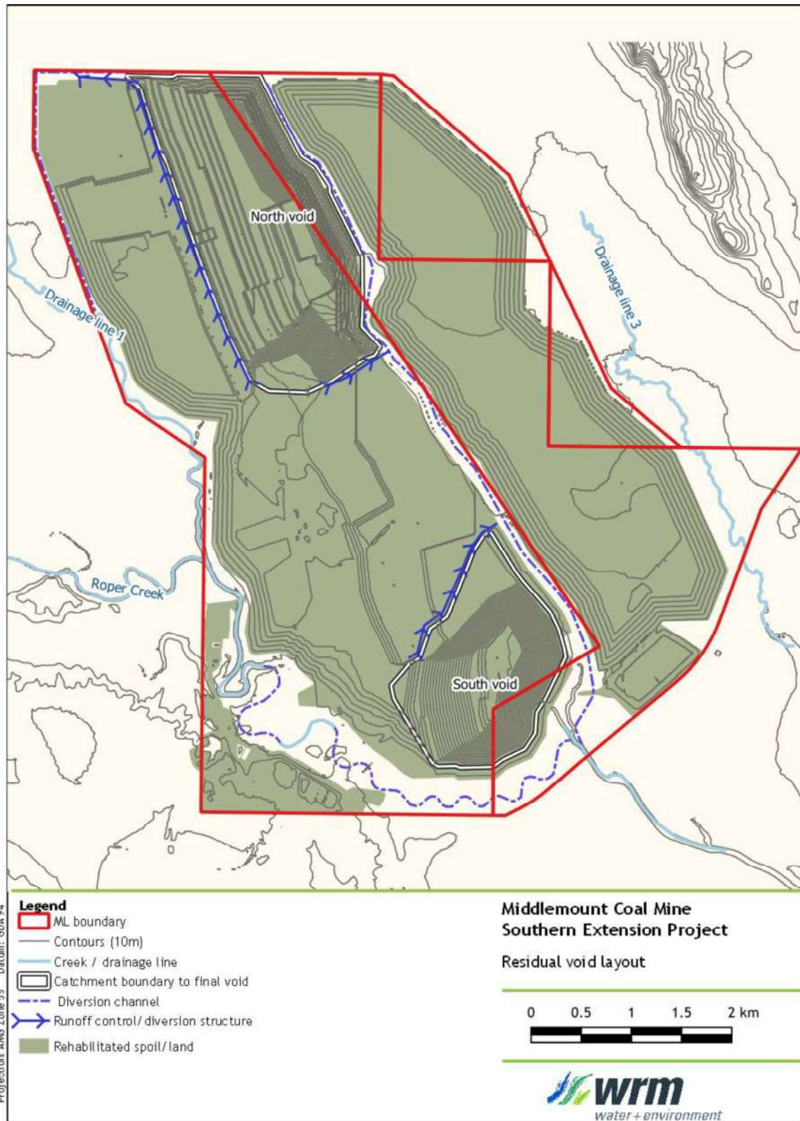
Figure 7.1 - Residual void catchment plan
