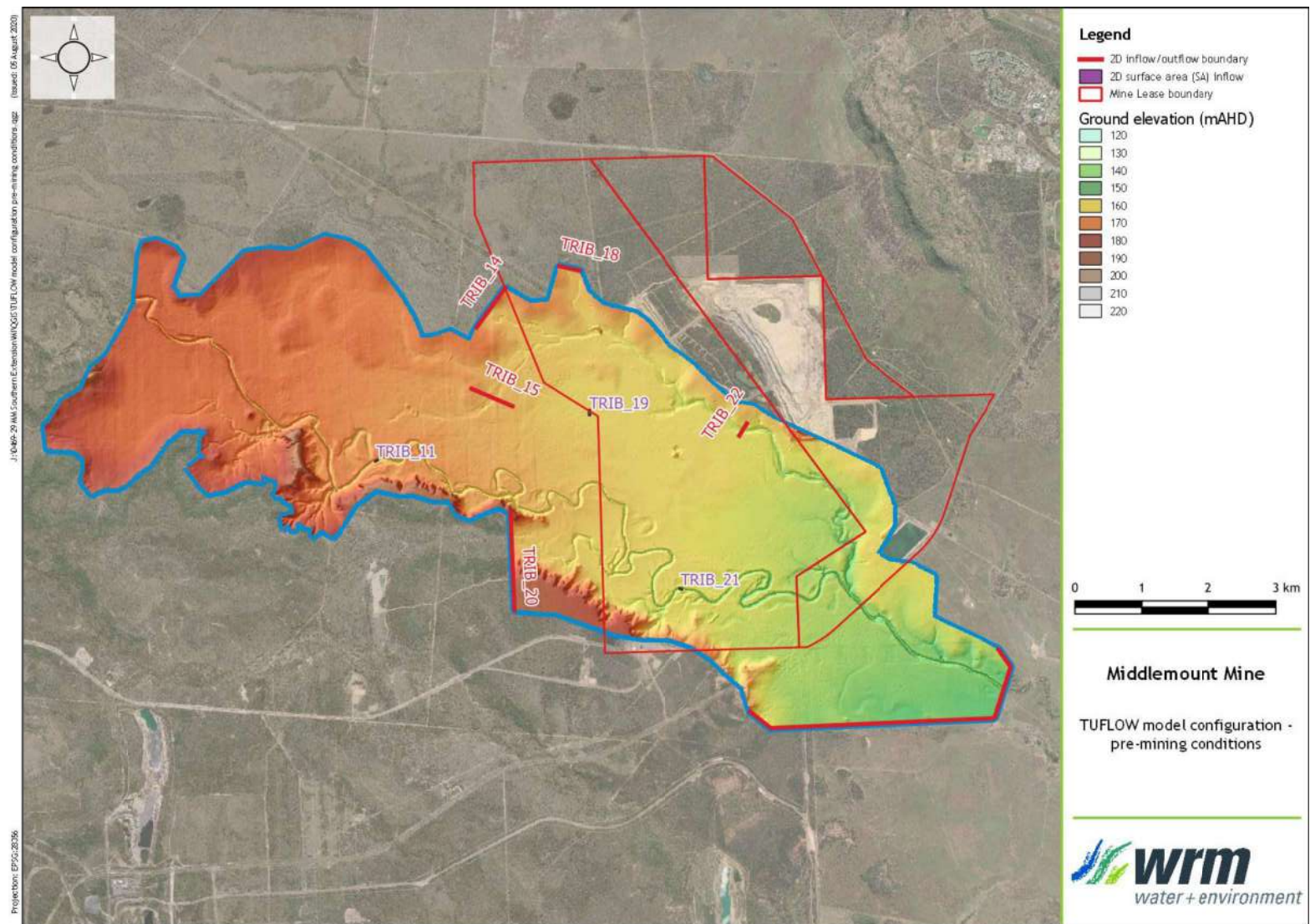
Figure 8.10 - Pre-mining Roper Creek TUFLOW model configuration
