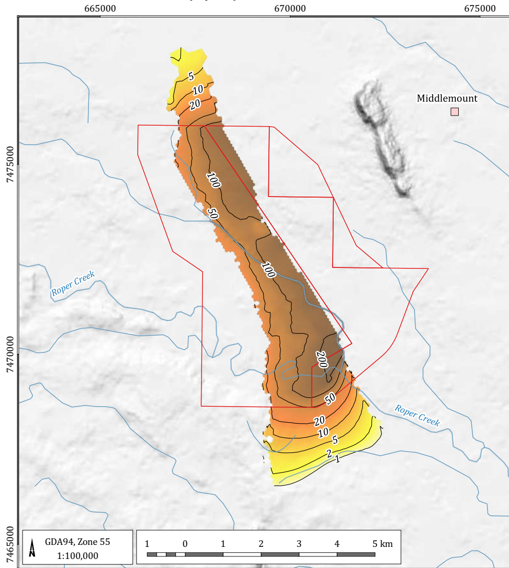
Maximum zone of drawdown - (Layer 5)
