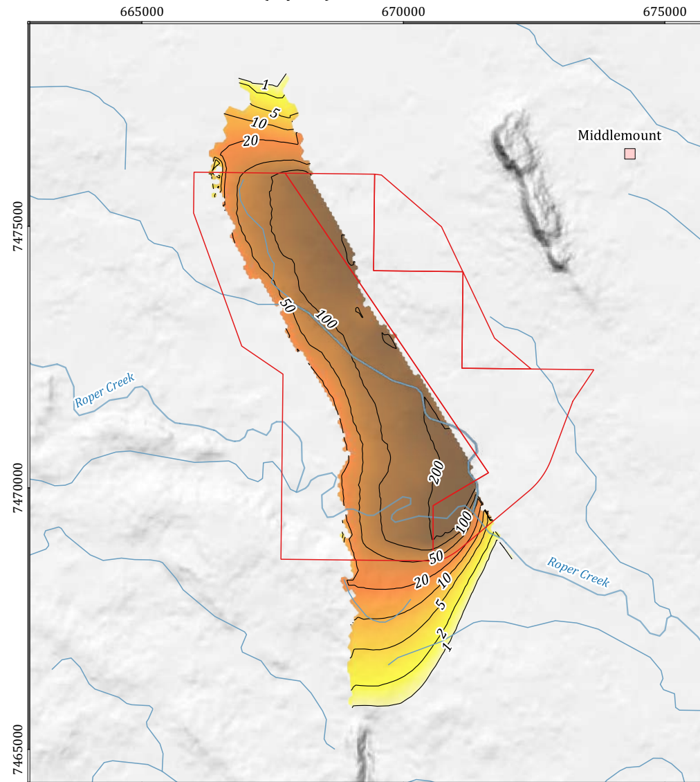
Maximum zone of drawdown - (Layer 7)
