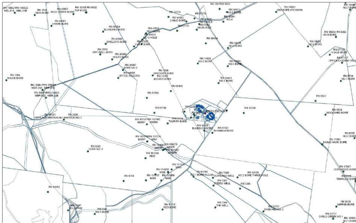
Figure 1: Draft map based on the 2012 DNRM database of registered groundwater bores.
