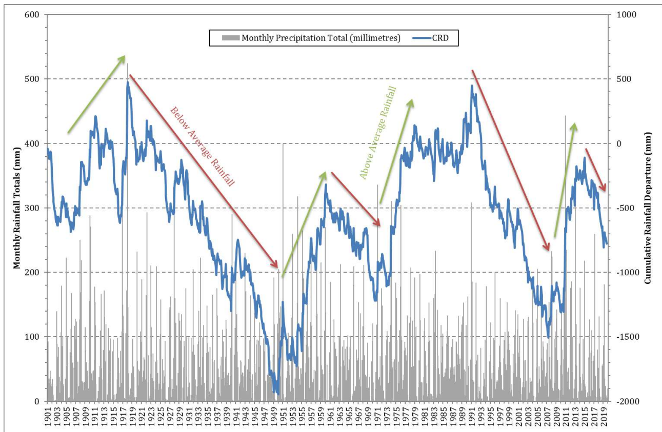
Figure 4.1 Monthly rainfall and cumulative rainfall departure – SILO Data for Middelmont Coal Mine 1901 to 2019
