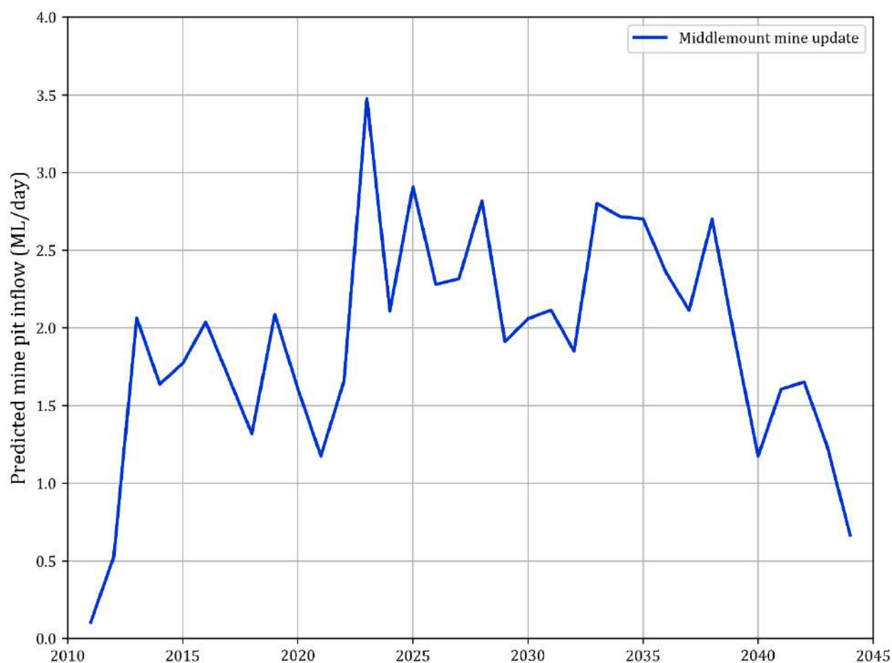
Figure 8.1 Predicted average annual pit inflows
