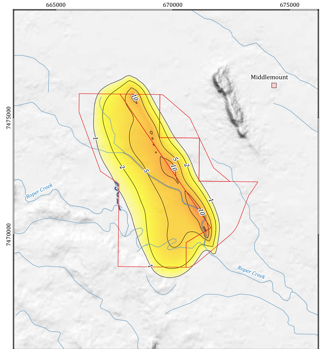
Maximum zone of drawdown (Layer-10 & 17)
