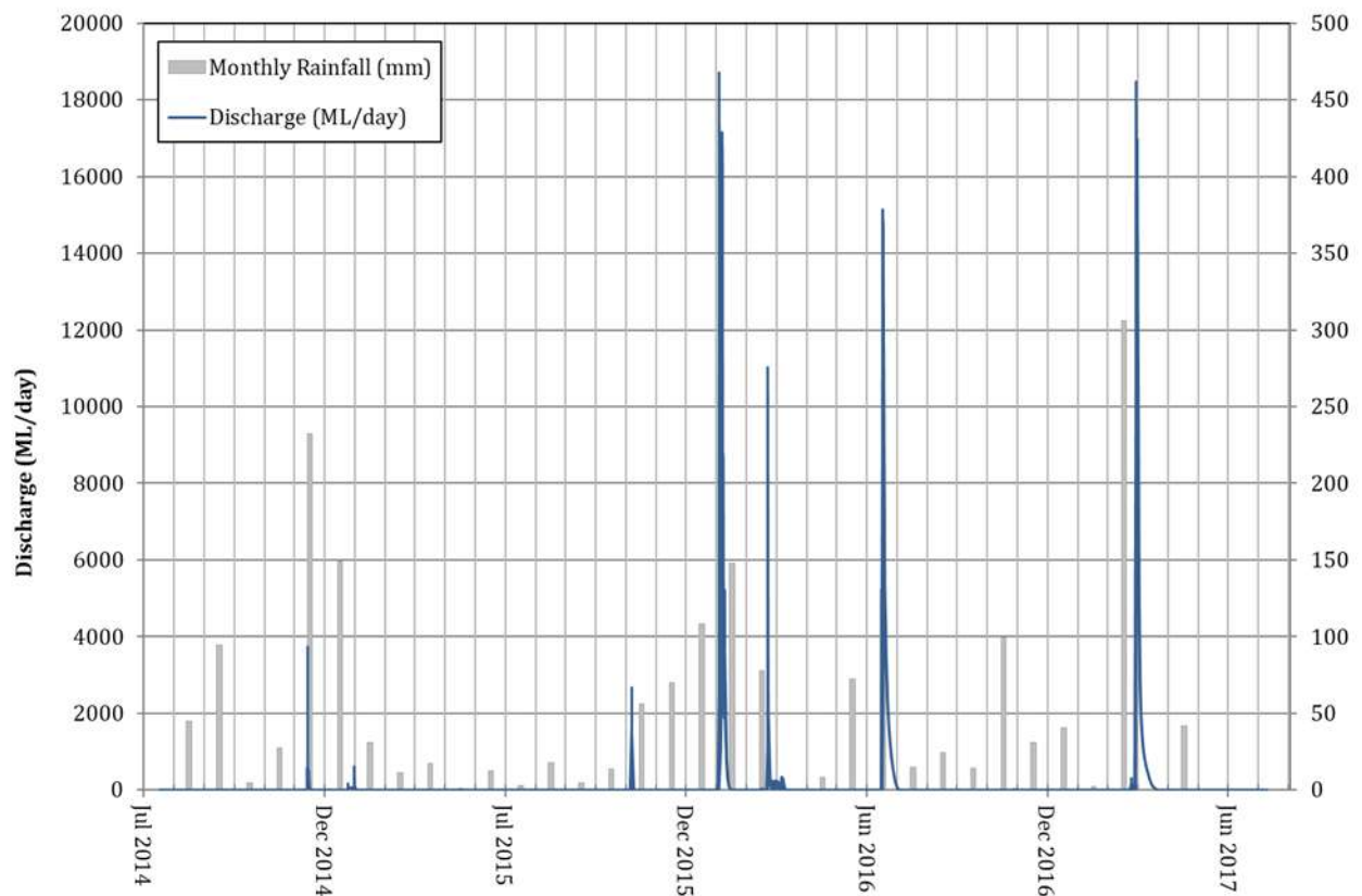
Figure 4.3 MCPL Roper Creek gauging station (Ref1)
