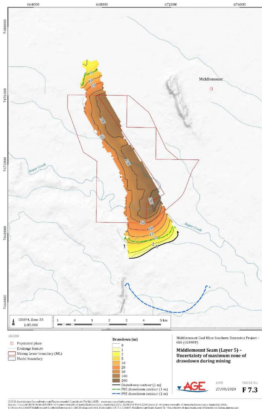
Figure F 7.3 Middlemount Seam (Layer 5) – Uncertainty of maximum zone of drawdown during mining
