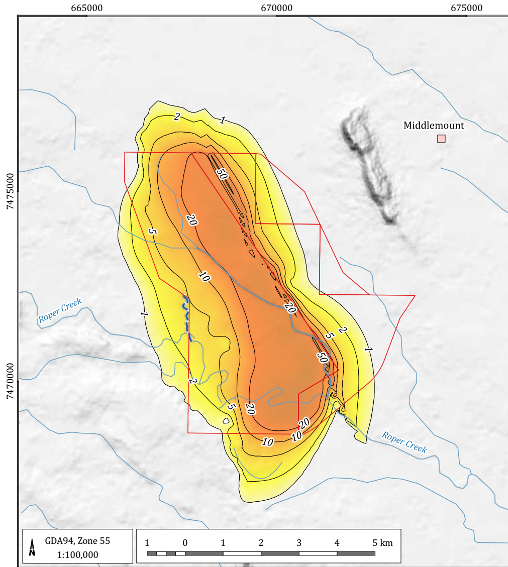
Maximum zone of drawdown (Layer-9 & 16)
